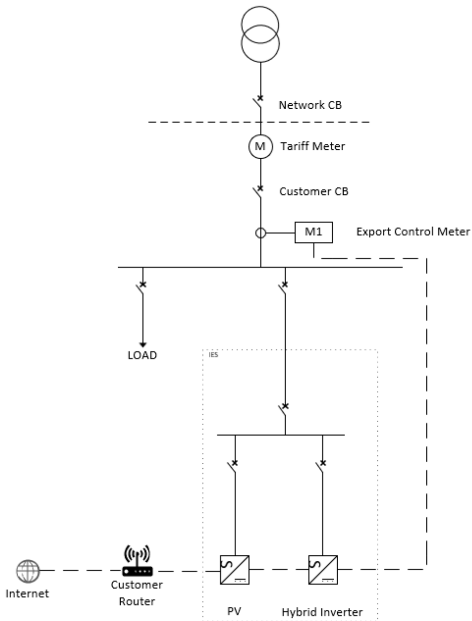
Figure 4: Typical single line diagram for IES system with compliant inverters
